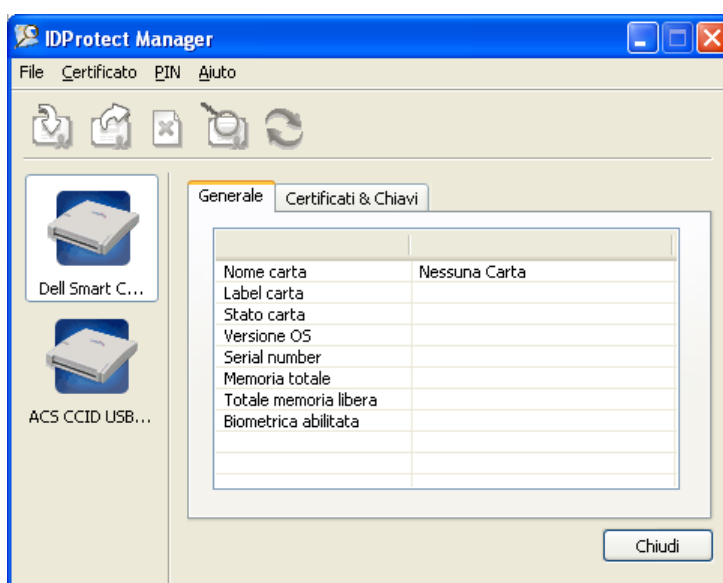
Figura 3: IDProtect Manager
